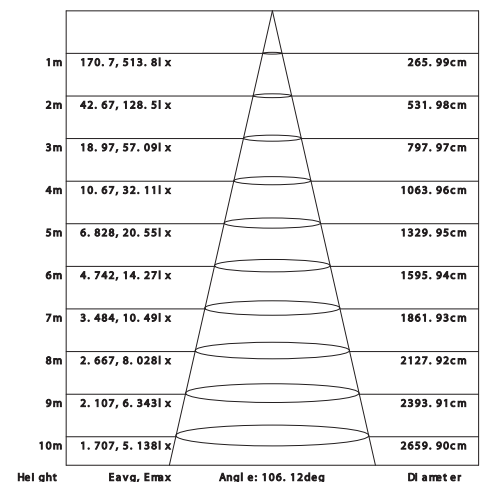
Beam angle
