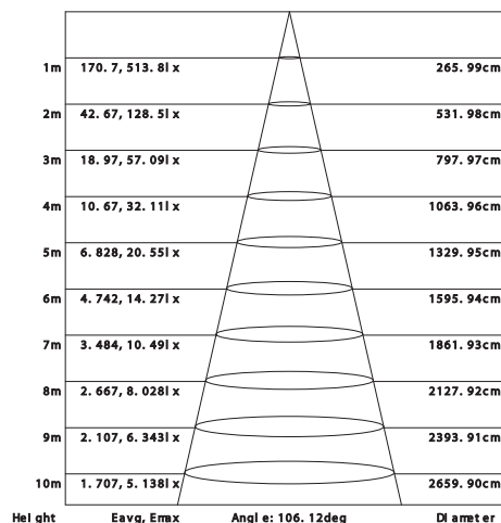
Beam angle
