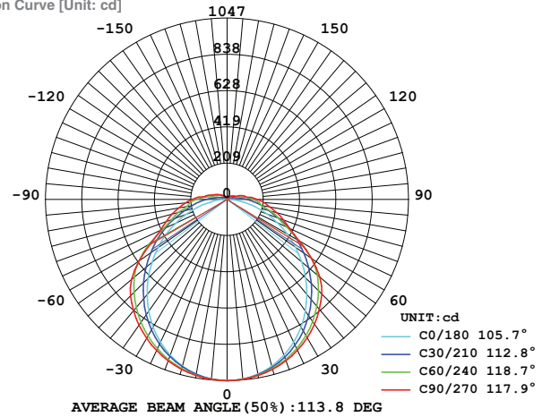
Light Distribution Curve [Unit: cd]
