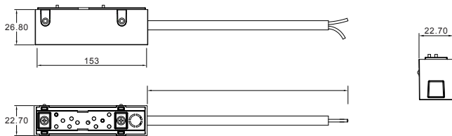
Power Connector
